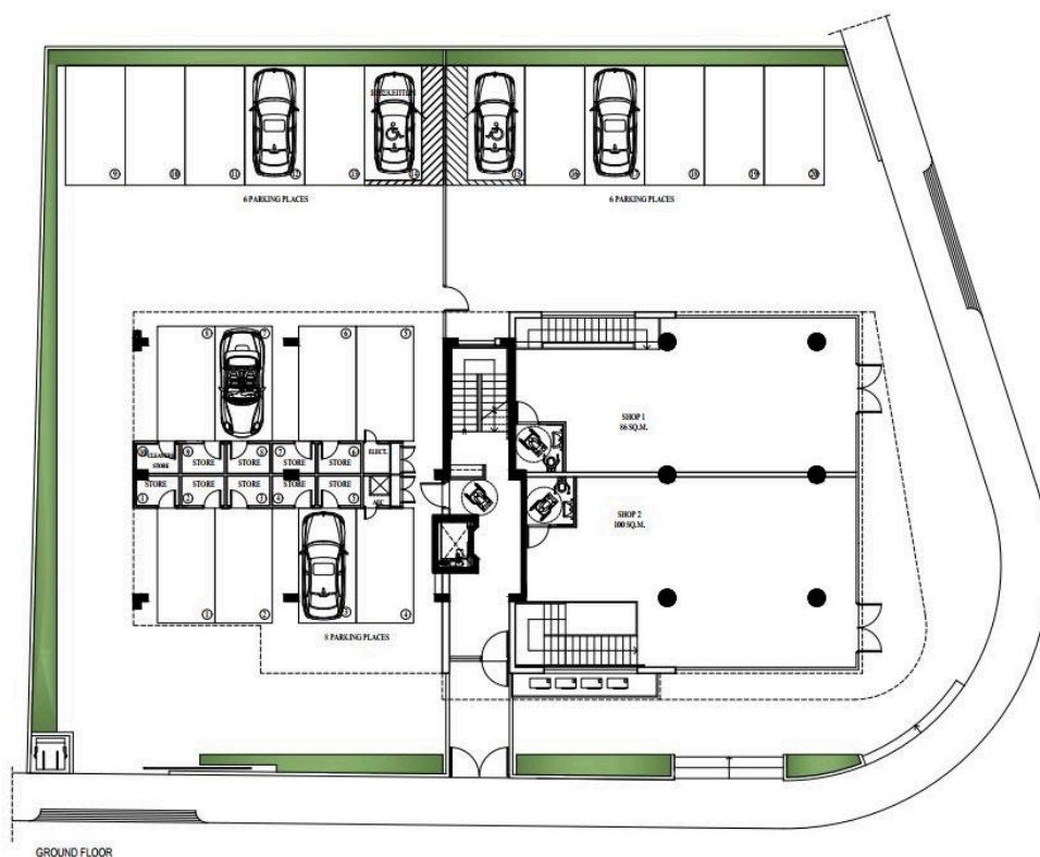
GROUND FLOOR
