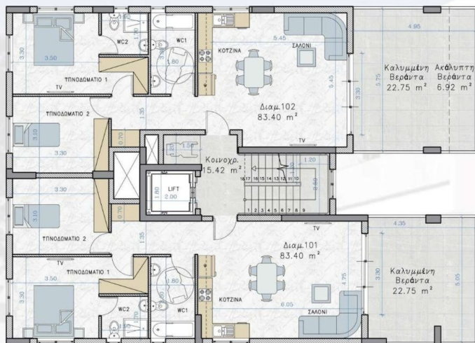
ΚΑΤΟΨΗ 1 ου & 3 ου ΟΡΟΦΟΥ
